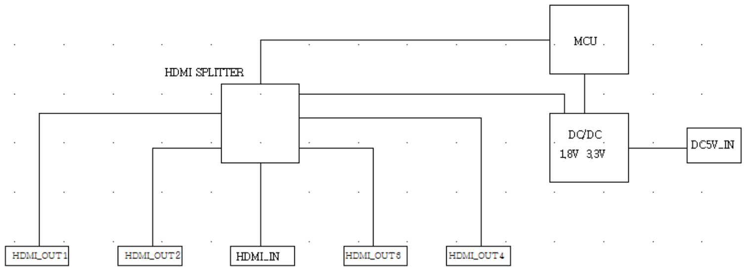
LKV314Pro block diagram
