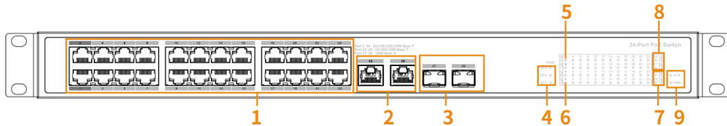
Figure 2-3 Front panel
